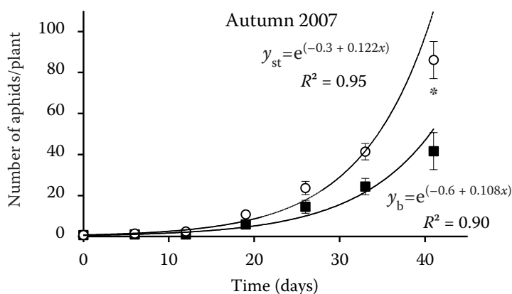
Fig. 1. Growth of M. euphorbiae population in the plots covered with a UV-absorbing net (Bionet: ■ —) and a Standard net (○ - - -). The growth model is shown by the equation [y = \exp(b_0 + b_1 t)] and the coefficient of determination ( R^2 ). An asterisk (*) shows differences between the nets at harvest
